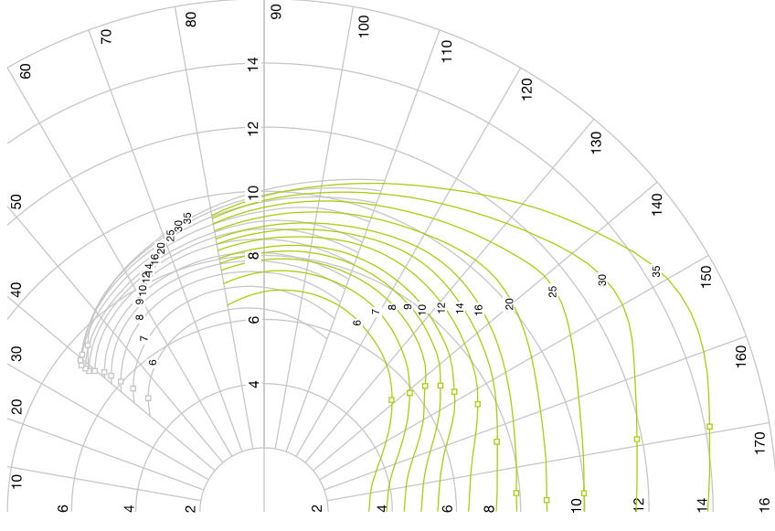
POLAR DIAGRAM
